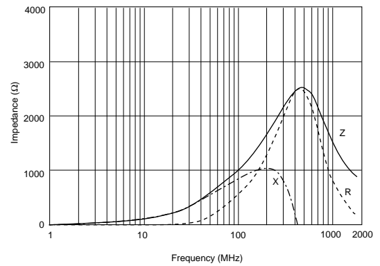
BLM18HD102SH1
