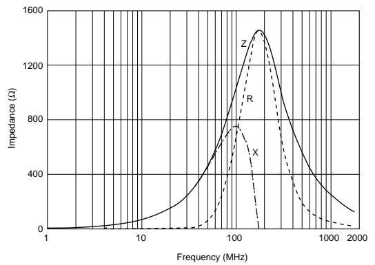
BLM15BD102SH1
