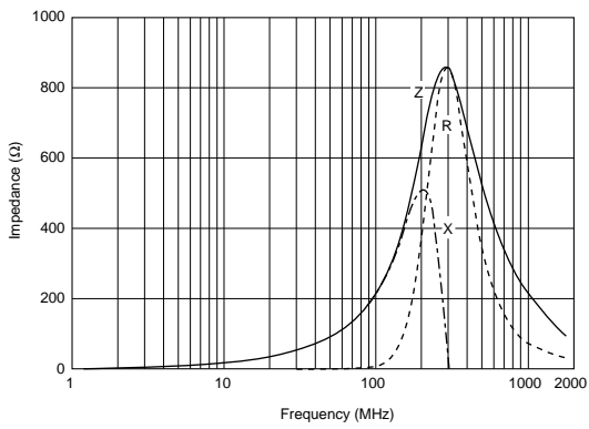
BLM21BB221SH1
