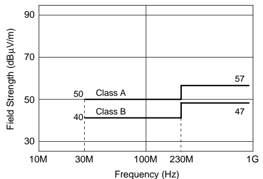
Radiated Interference
